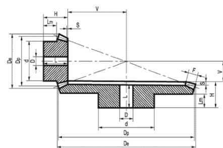
Type B Pressure angle 20° Ratio 1:4
