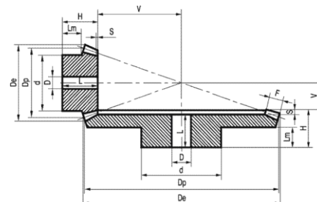
Type B Pressure angle 20° Ratio 1:3
