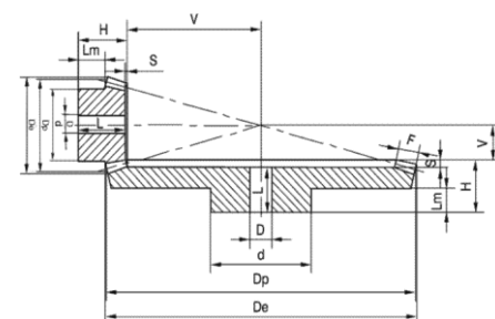
Type A Pressure angle 20° Ratio 1:4
