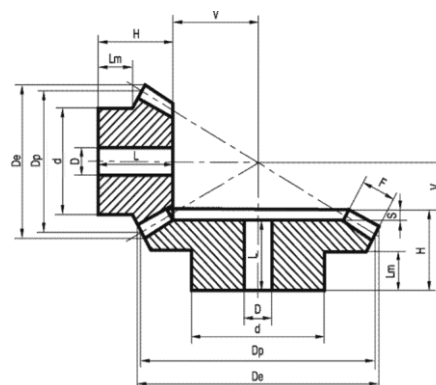
Type B Pressure angle 20° Ratio 1:2
