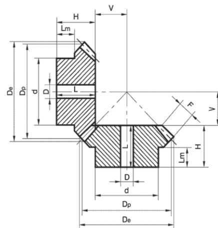
Type B Pressure angle 20° Ratio 1:1
